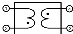
Figure 1. Electrical Schematic
